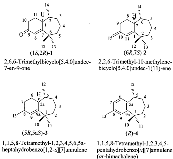
Figure 1. Structures of Aphthona flava himachalenes; nomenclature is adopted to Chemistry 4-D Draw ver. 5.0 (Chem. Innovation Software, Inc.)
