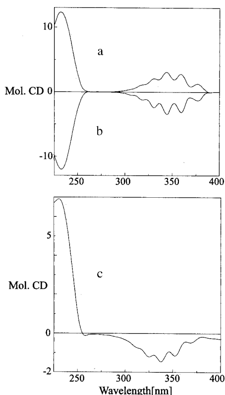
Figure 3. CD spectra of (a) (1 R ,2 S )-(-)-1 (1.63 mm in hexane); (b) (1 S ,2 R )-(+)-1 (1.33 mm in hexane); and (c) cholest-4-en-3-one (1.67 mm in hexane)
