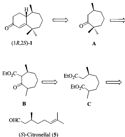
Scheme 1. Retrosynthetic analysis of (1 R ,2 S )- 1
