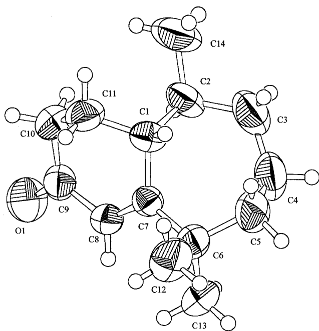
Figure 2. X-ray structure of (1 R ,2 S )-(-)-1
