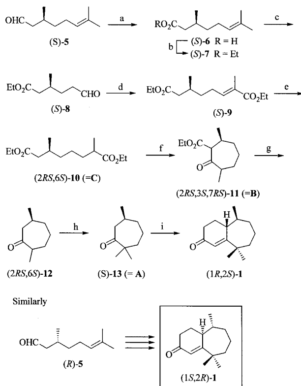
Scheme 2. Synthesis of 1 ; reagents and conditions: (a) PDC, DMF, 0 °C to room temp.; (b) K 2 CO 3 , EtI, DMF, 0 °C to room temp. (74%, 2 steps); (c) O 3 , MeOH, –78 °C; then Me 2 S (72%); (d) (EtO) 2 P(O)CHMeCO 2 Et, NaH, THF, –30 °C (96%); (e) H 2 , PtO 2 , EtOAc, room temp. (quant.); (f) i) t BuOK, m -xylene, 150 °C; ii) diluted HCl (79%); (g) i) NaOH, MeOH, H 2 O, reflux; ii) diluted HCl (85%); (h) t BuOK, t BuOH, MeI, 0 °C to room temp. (88% based on consumed 12 ); (i) LDA, TMSCl, THF, –78 °C; ii) MeLi, CH 2 =C(TMS)COMe, THF; iii) NaOMe, MeOH, room temp. (44% based on consumed 13 )
