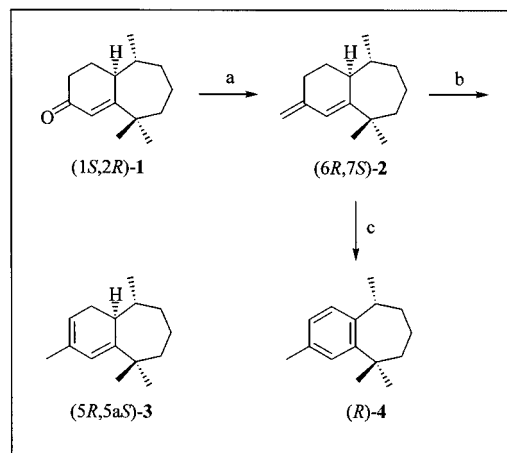
Scheme 3. Synthesis of 2 , 3 and 4 ; reagents and conditions: (a) \text{Ph}_3\text{PMeBr} , n\text{BuLi} , THF, 0 °C to room temp. (69% based on consumed 1 ); (b) \text{HCO}_2\text{H} , MeOH, room temp. (88% based on consumed 2 ); (c) chloranil, \text{C}_6\text{H}_6 , 75 °C (63%)
